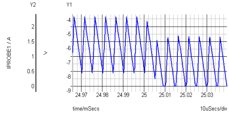
Fig.8 Waveform of inductor current
