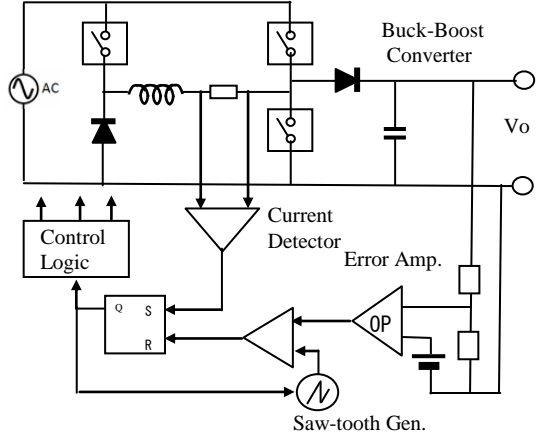
Fig.16 New BCM PFC without an analog multiplier.
