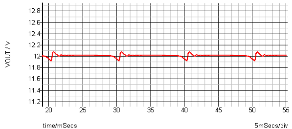
Fig.12 Output ripple of the inverting converter
