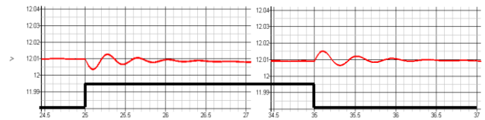
Fig.13 Load transient response
