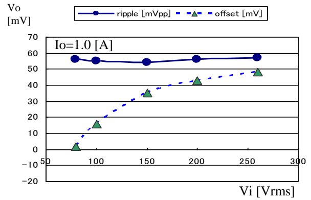
Fig.22 Output ripple and offset vs. input voltage
