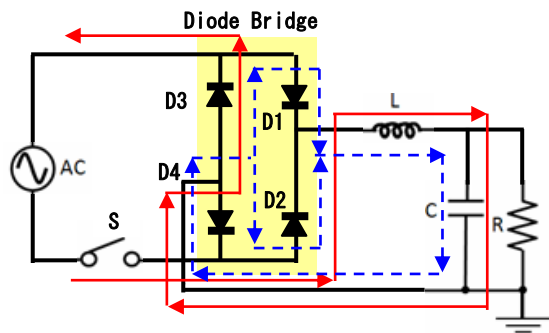
(b) Current flow when V_i < 0
