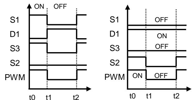
(a) V_{in} > 0 (b) V_{in} < 0 Fig.3 Timing chart of switches
