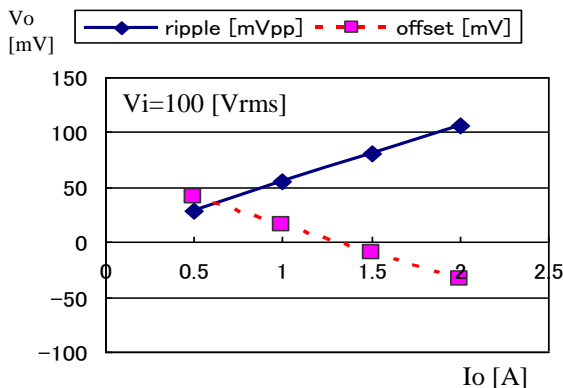
Fig.21 Output ripple and offset vs. output current
