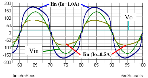
Fig.17 Waveform of V_i , V_o and I_{in} (through LPF)
