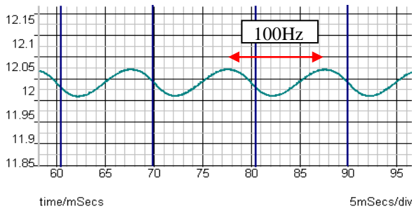
Fig.18 Output voltage ripple ( I_o=1.0 A).
