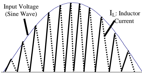
Fig.15 Waveform of inductor current in BCM.
