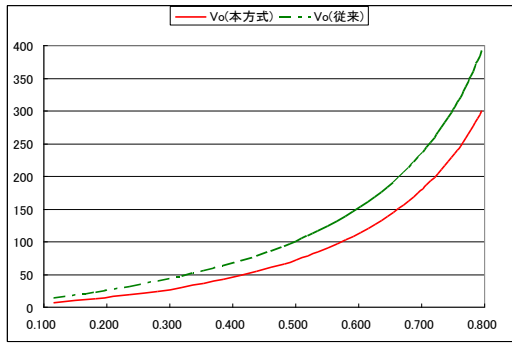
Fig.9 Average duty ratio vs. V_o ( V_i rms=100V)
