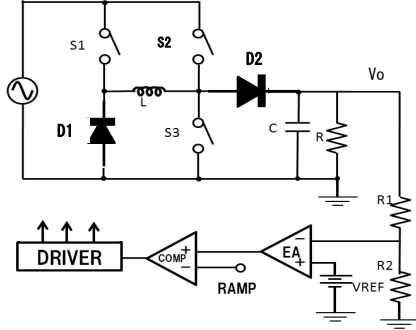
Fig.4 Simulation circuit
