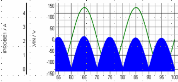
Fig.19 Input voltage and inductor current.
