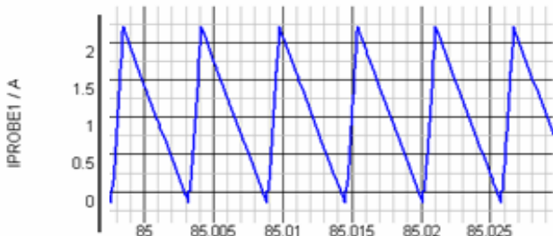
Fig.20 Inductor current in BCM.
