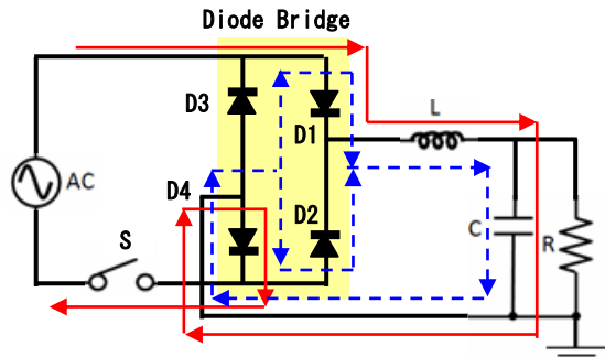
(a) Current flow when V_i > 0
