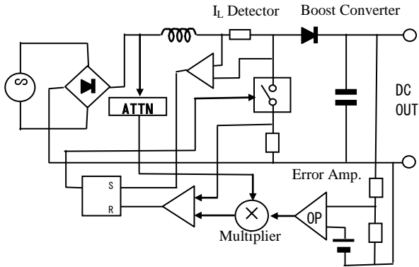
Fig.14 Conventional PFC circuit in BCM
